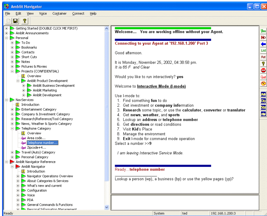
Amblit Navigator Main Screen
